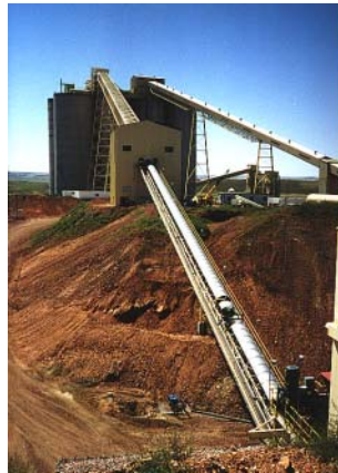
Jacob's Ranch, Wyoming; 6,000 TPH Conveyor Belts
